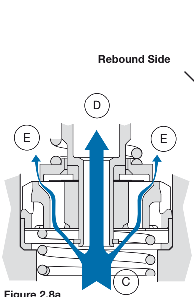
Figure 2.8a Flow through the main valve TTX40 MkII.
