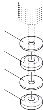
Figure 23.1 Example of a bump rubber stack.
