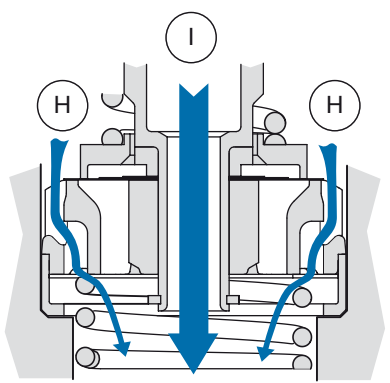
Figure 2.8b Flow through the check valve TTX40 MkII.
