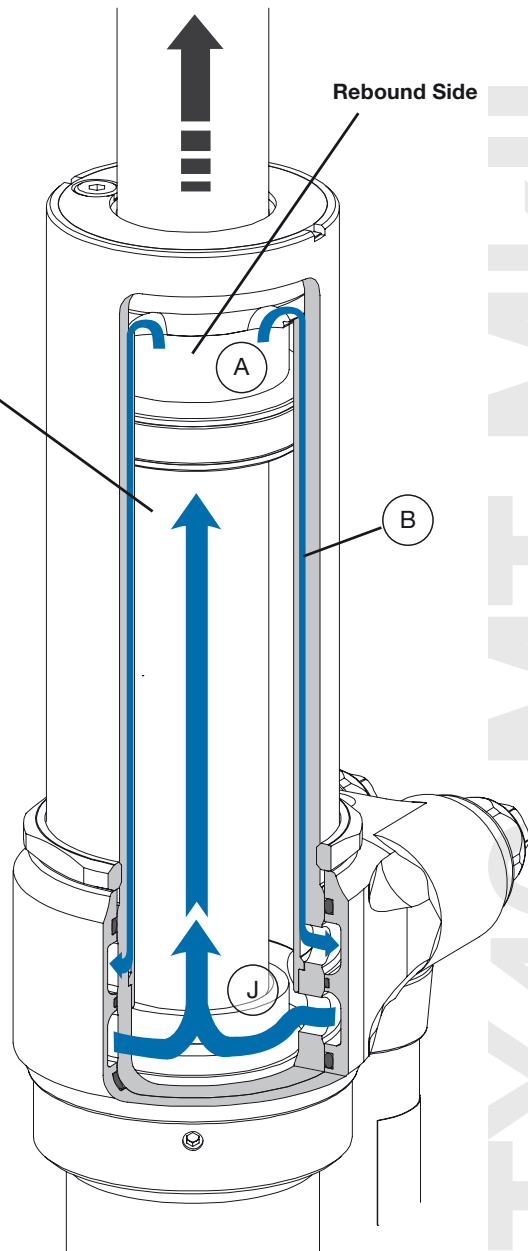
Figure 2.13 Flow circuit during rebound cycle for TTX46 MT MkII.
