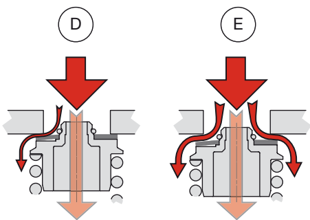
Figure 2.2 Poppet valve for compression TTX40 Mkl.
