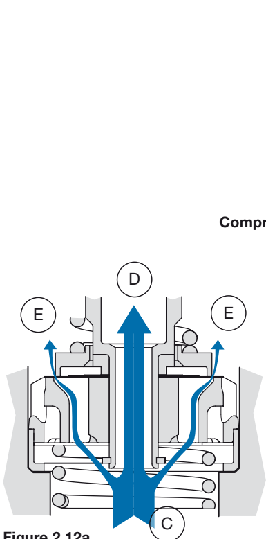
Figure 2.12a Flow through the main valve TTX46 MT MkII.
