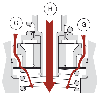
Figure 2.10b Flow through the check valve TTX46 MT MkII.
