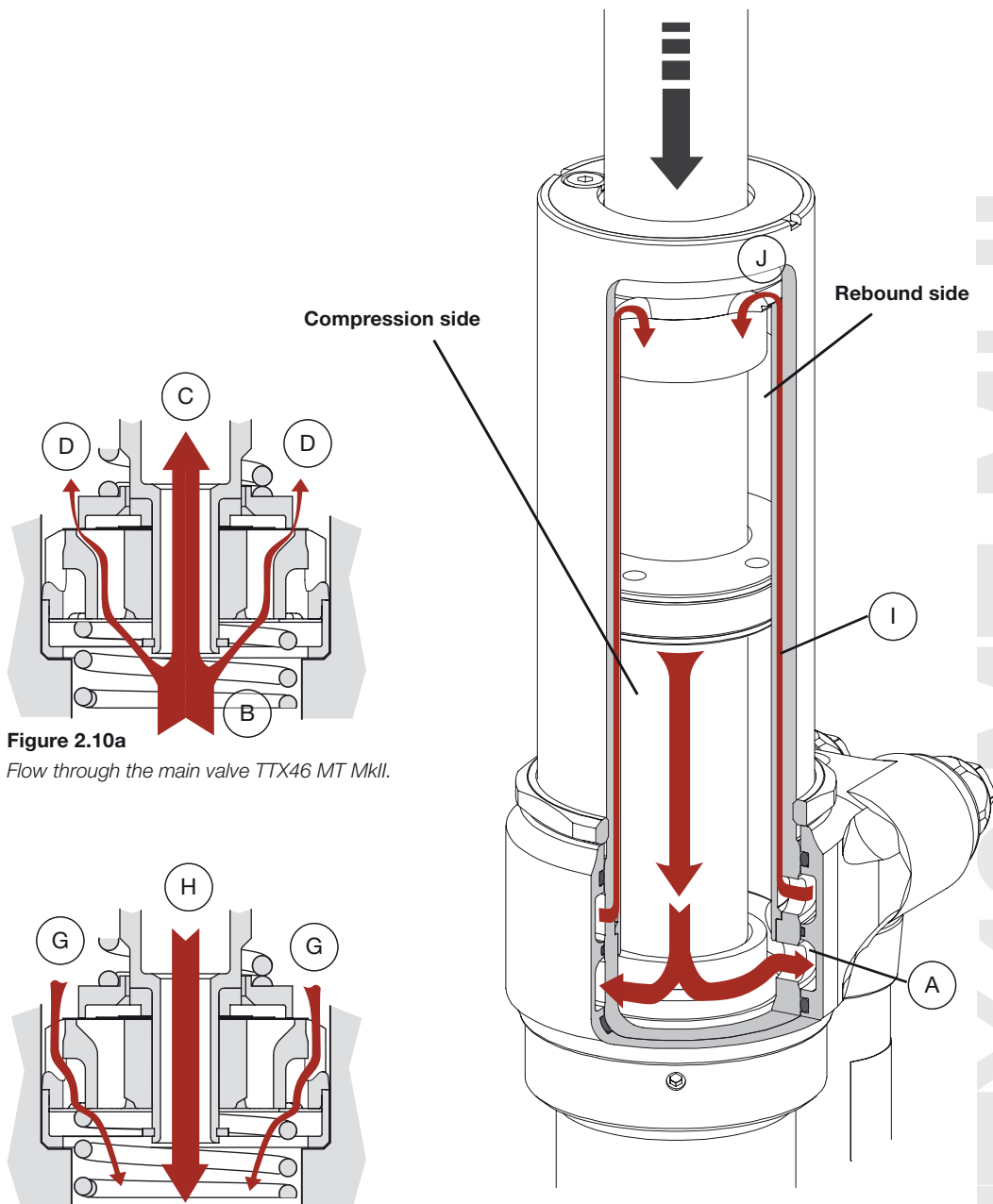
Figure 2.10b Flow through the check valve TTX46 MT MkII.
