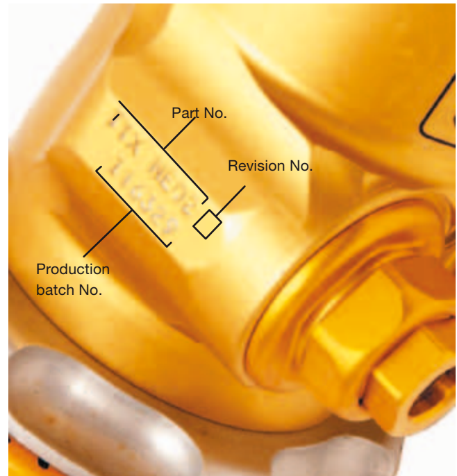
Figure 21.1 Damper identification.
