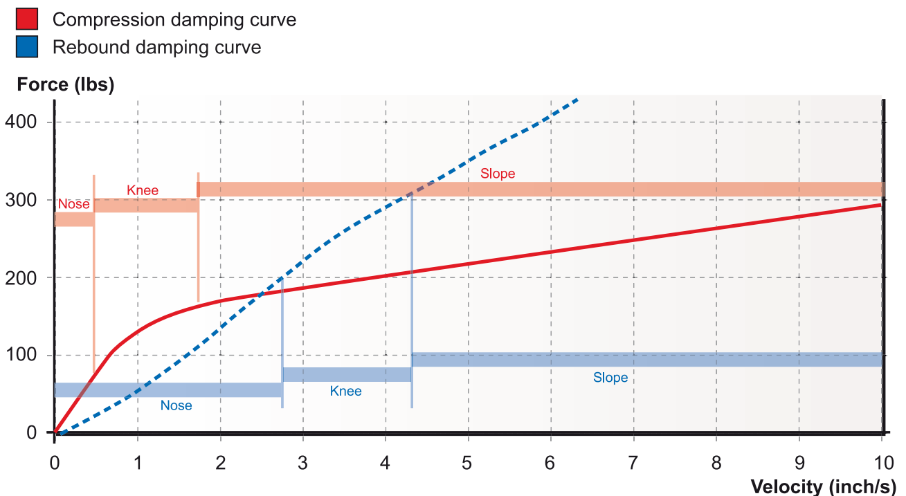
Figure 4.1 Terminology
