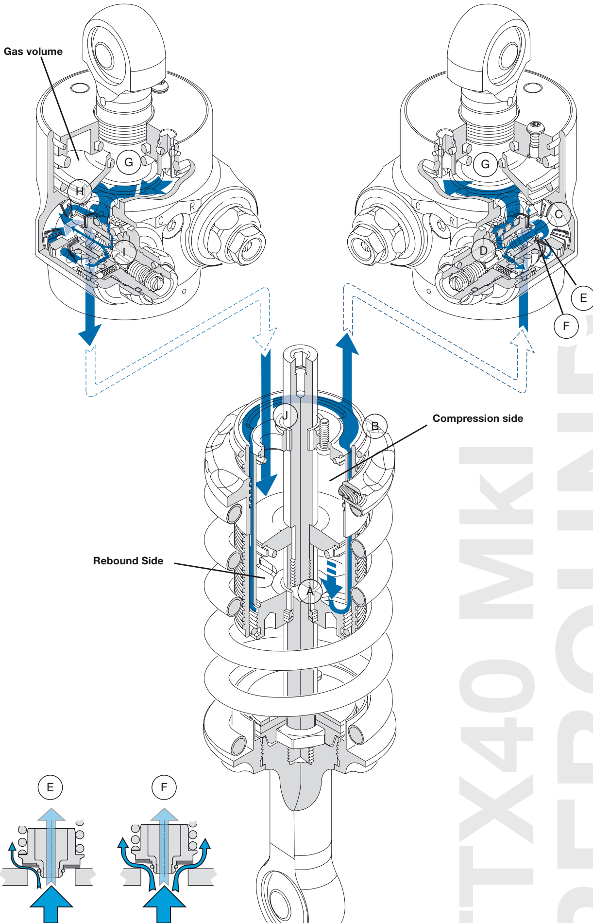
Figure 2.4 Poppet valve for rebound TTX40 Mkl.
