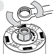
Spring preload adjuster
