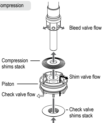
Fig. 3 - Piston Oil Flow
