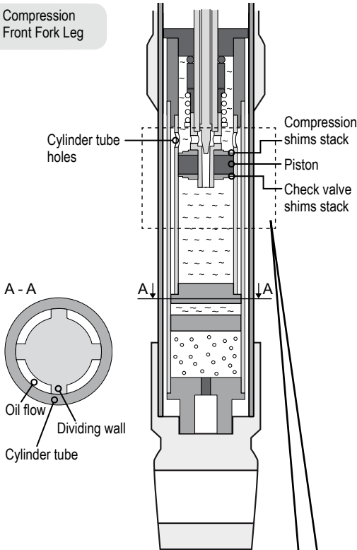
Fig. 3 - Piston Oil Flow
