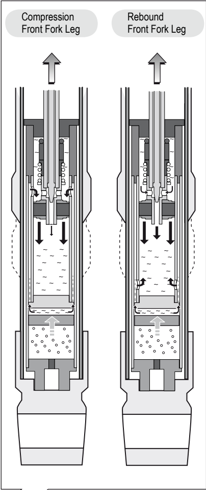
Fig. 5 - Front Fork Oil Flow Rebound Movement
